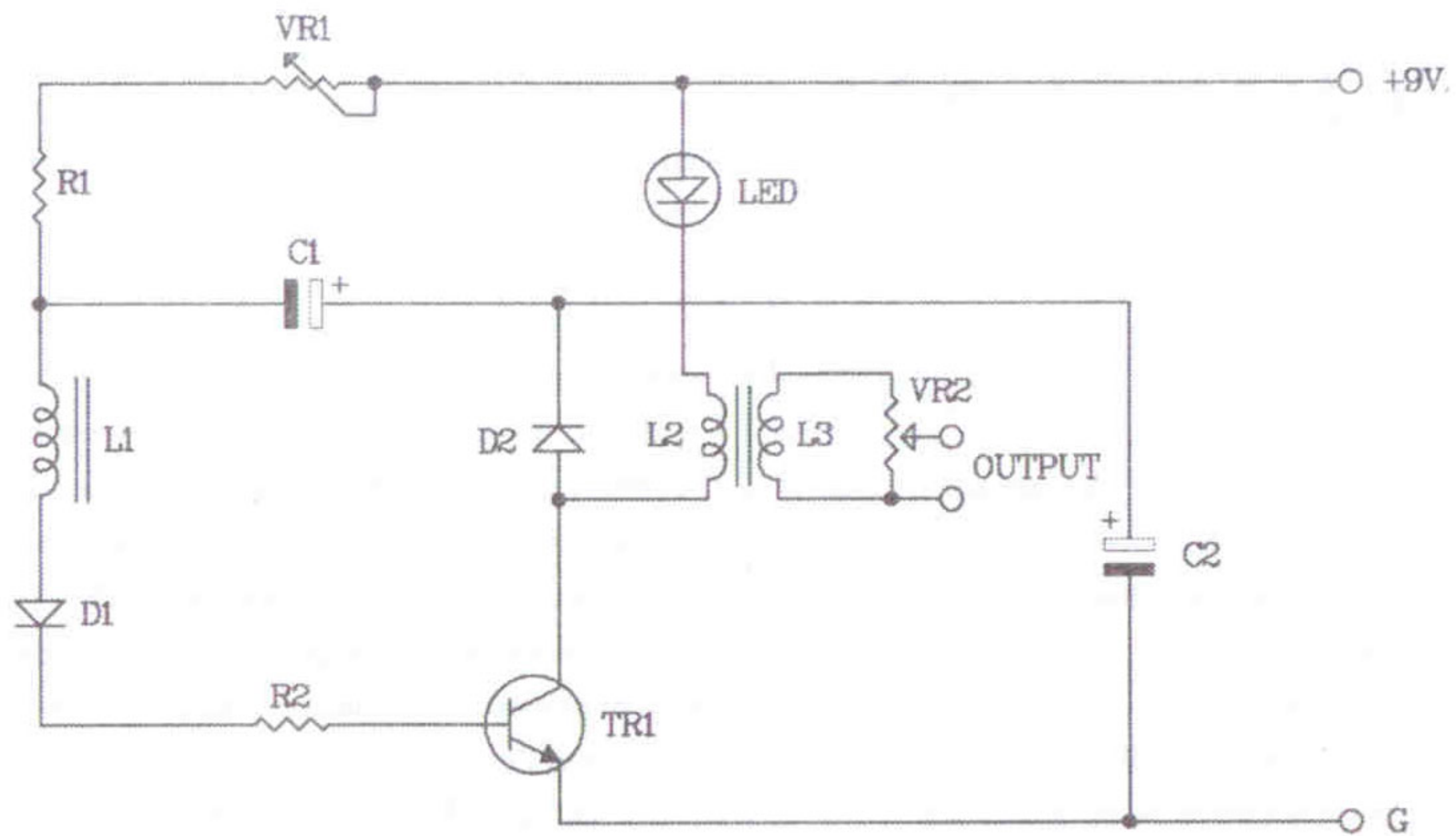
Figure 2. The muscle massage equipment circuit
