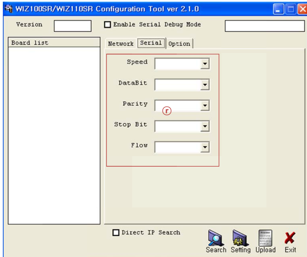
Figure 9. Configuration Tool 초기화면(Serial Config.)
