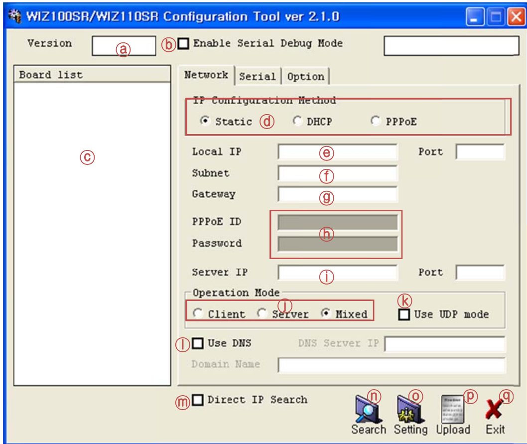
Figure 4. Configuration Tool 초기화면 (Network Config)
