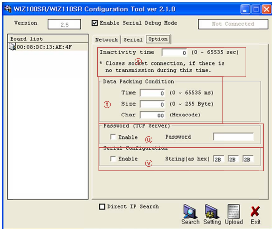
Figure 10. Configuration Tool 초기화면(OPTION Config.)
