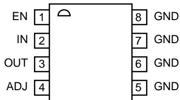
MIC5219BMM MM8™ MSOP-8 Adjustable Voltage
