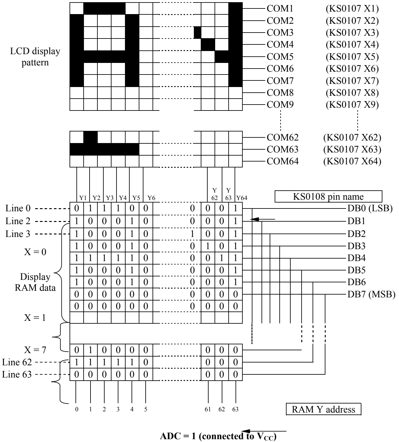
Relation between RAM Data and Display
