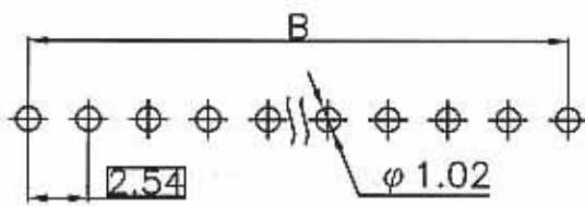
RECOMMEND P.C.B. LAYOUT BOTTOM VIEW
