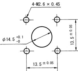
Mounting Hole
