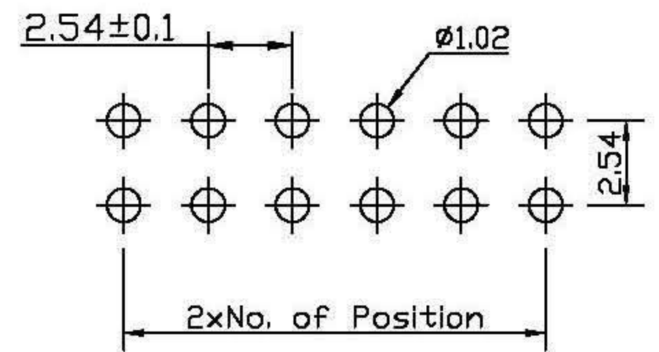
Recommended P.C.B Hole Layout
