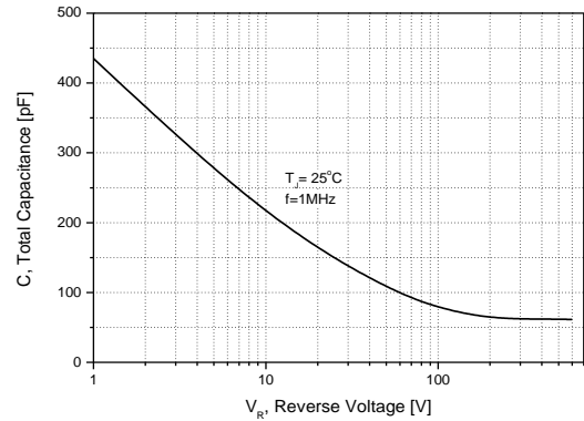
Figure 8. Total Capacitance
