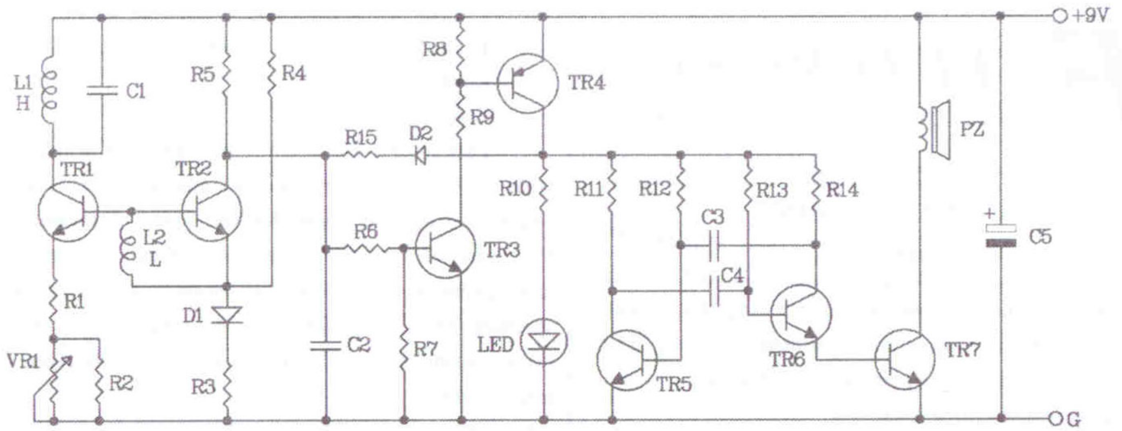
Figure 2. The metal detecting circuit
