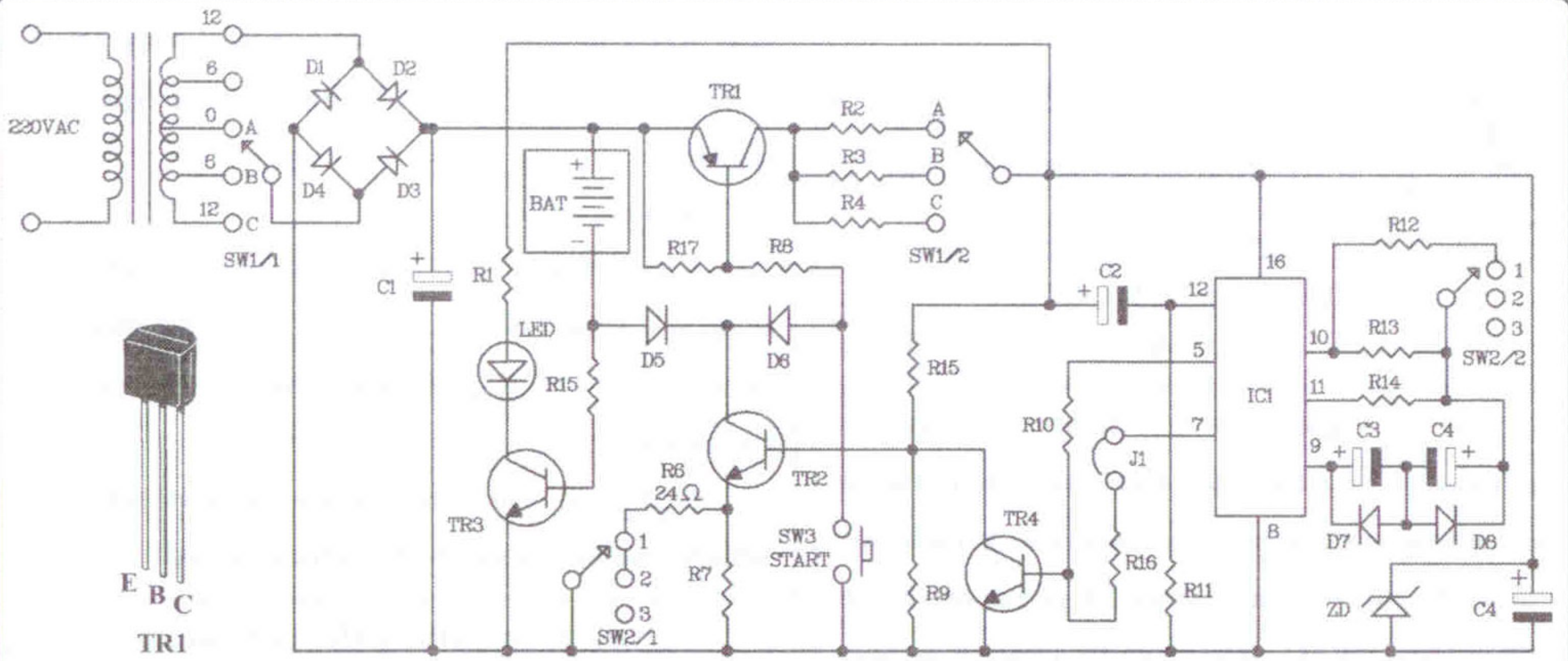
Figure 2. Automatic "Ni-Cd" charger circuit
