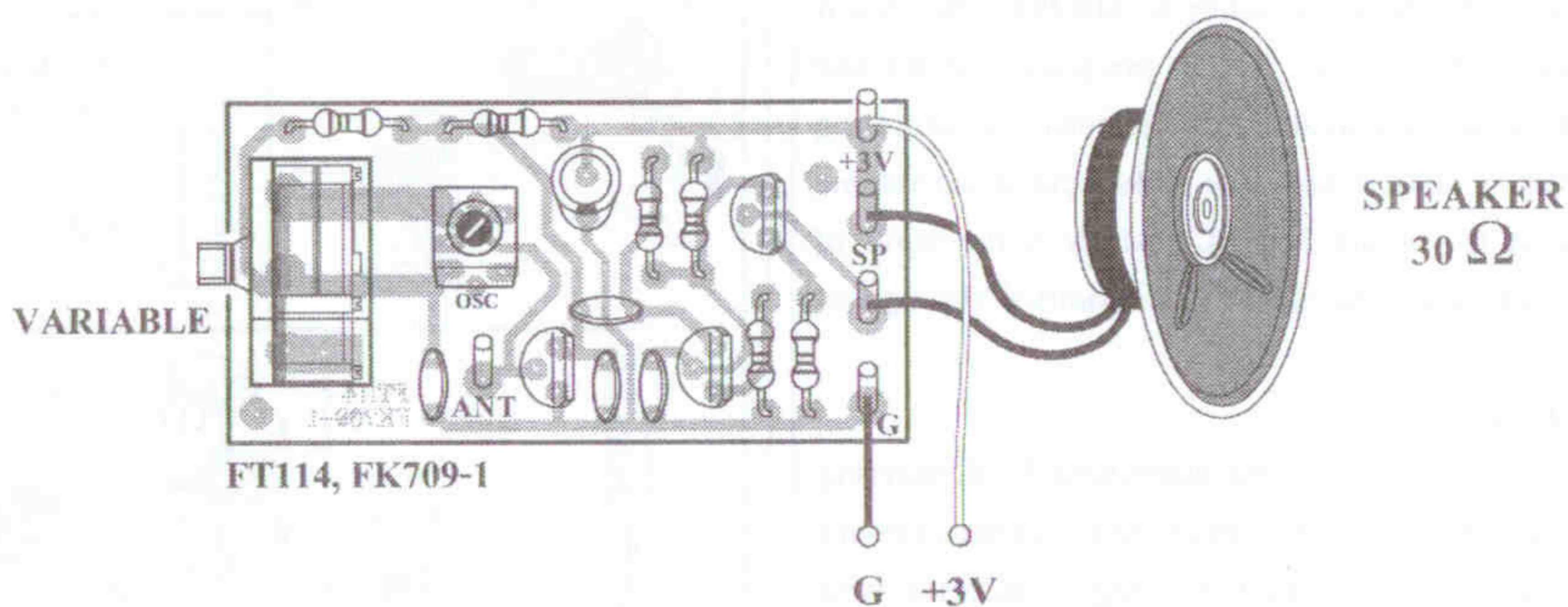
Figure 3. Connections
