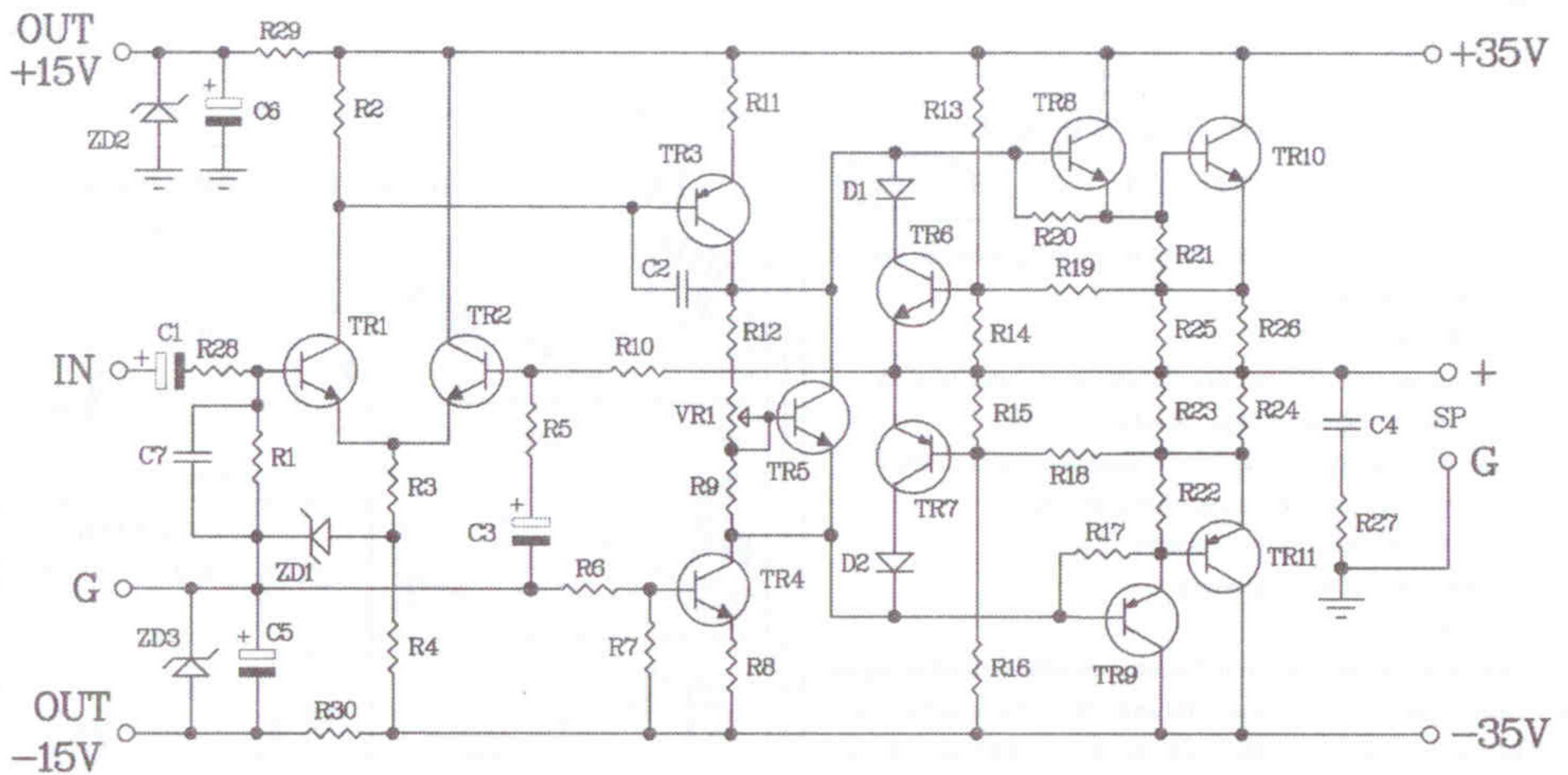
Figure 2. The power amp OCL 35W R1% circuit
