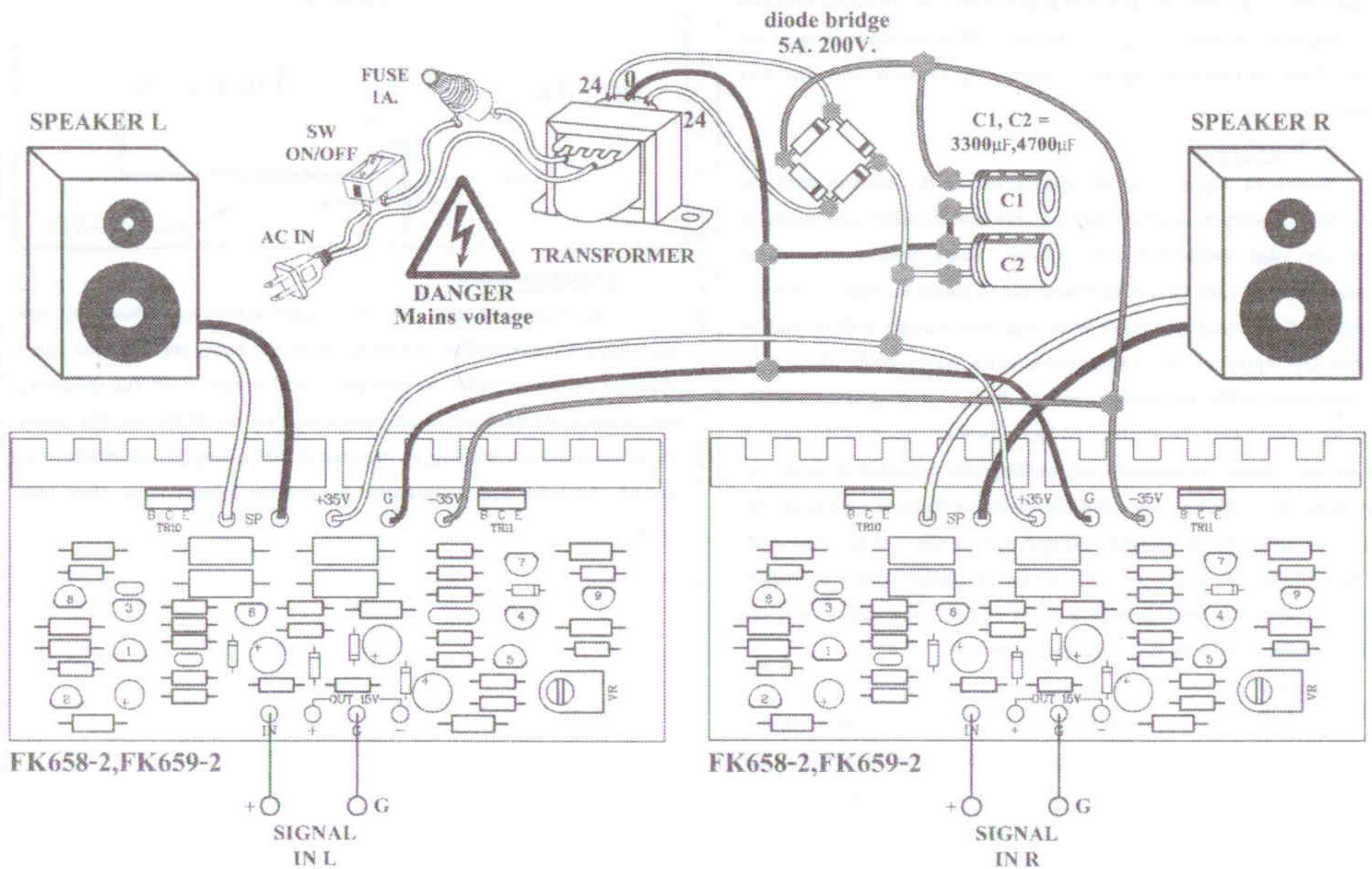
Figure 3. Connections
