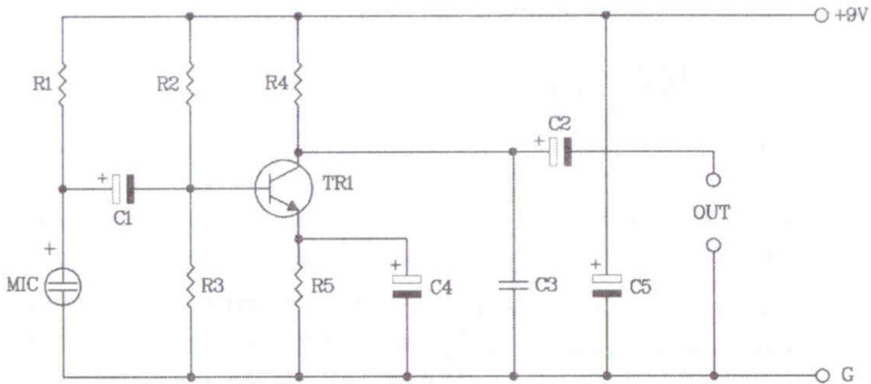
Figure 2. The condenser mic with pre-amp circuit
