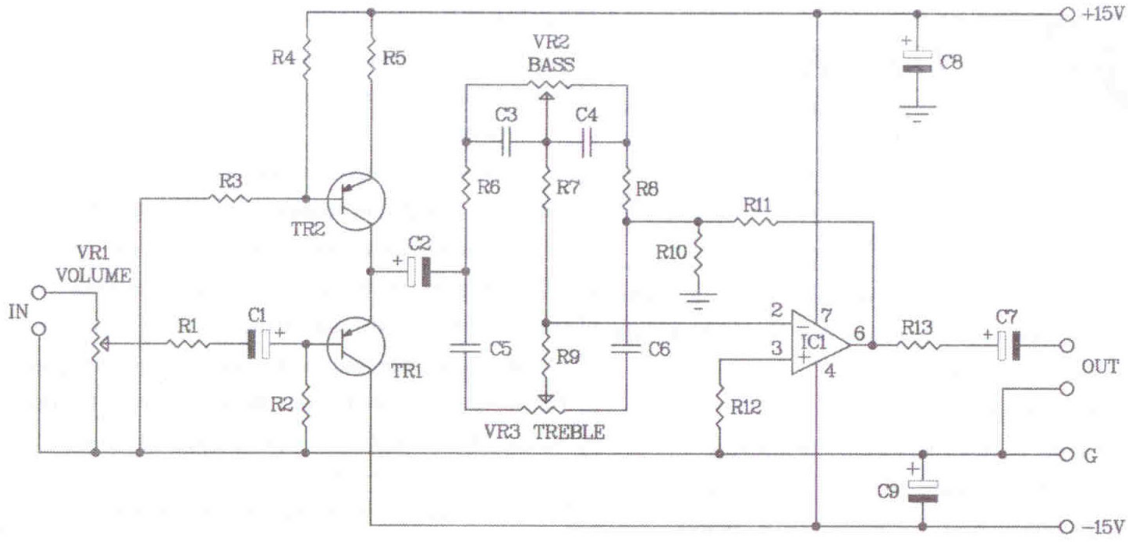
Figure 2. The super tone control (mono) circuit
