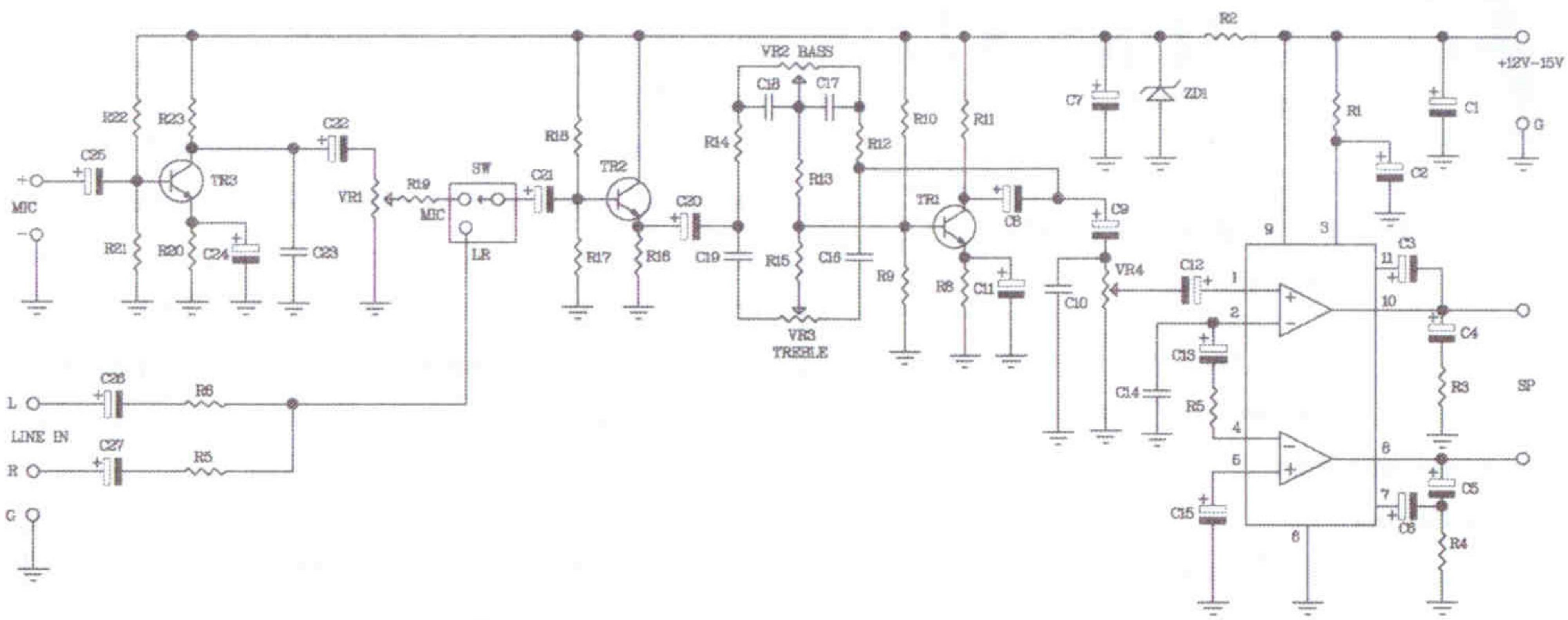
Figure 2. The power amplifier for teacher circuit
