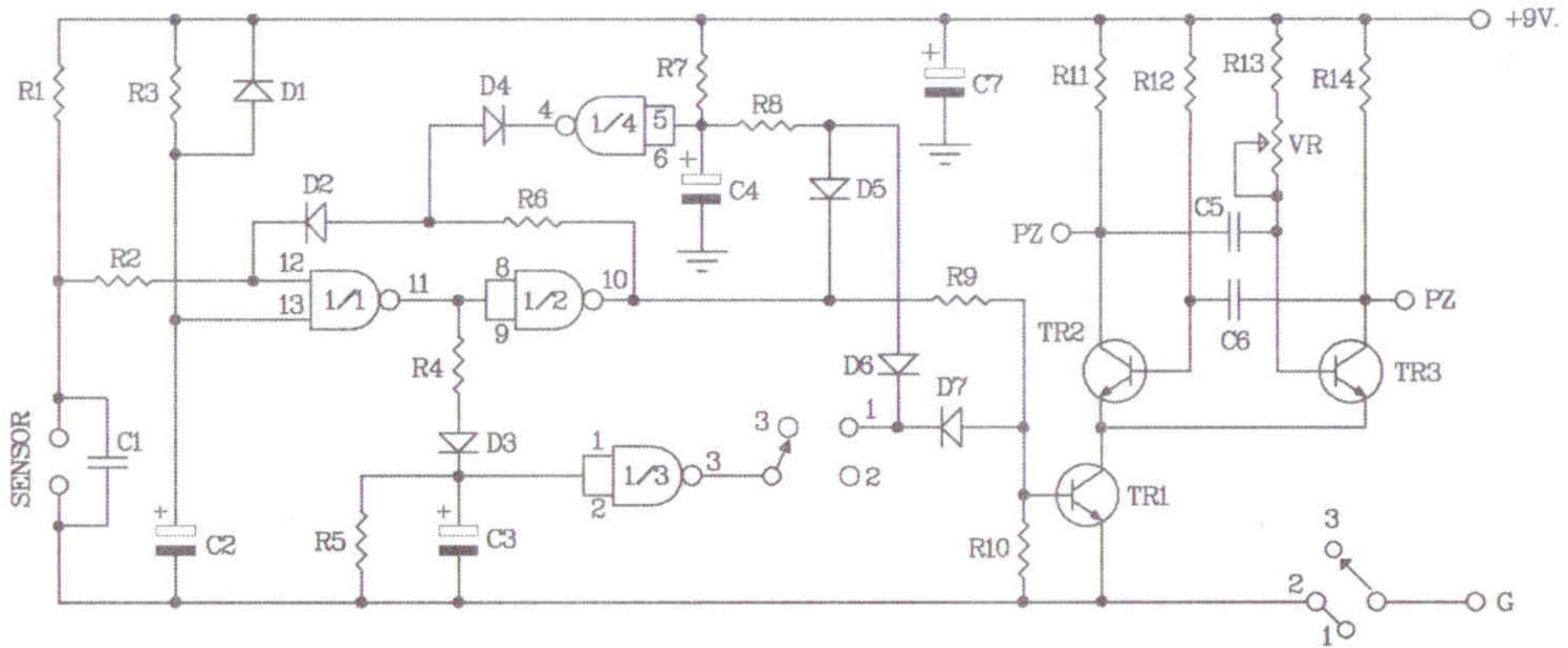
Figure 2. The magnetic sensor burglar alarm circuit
