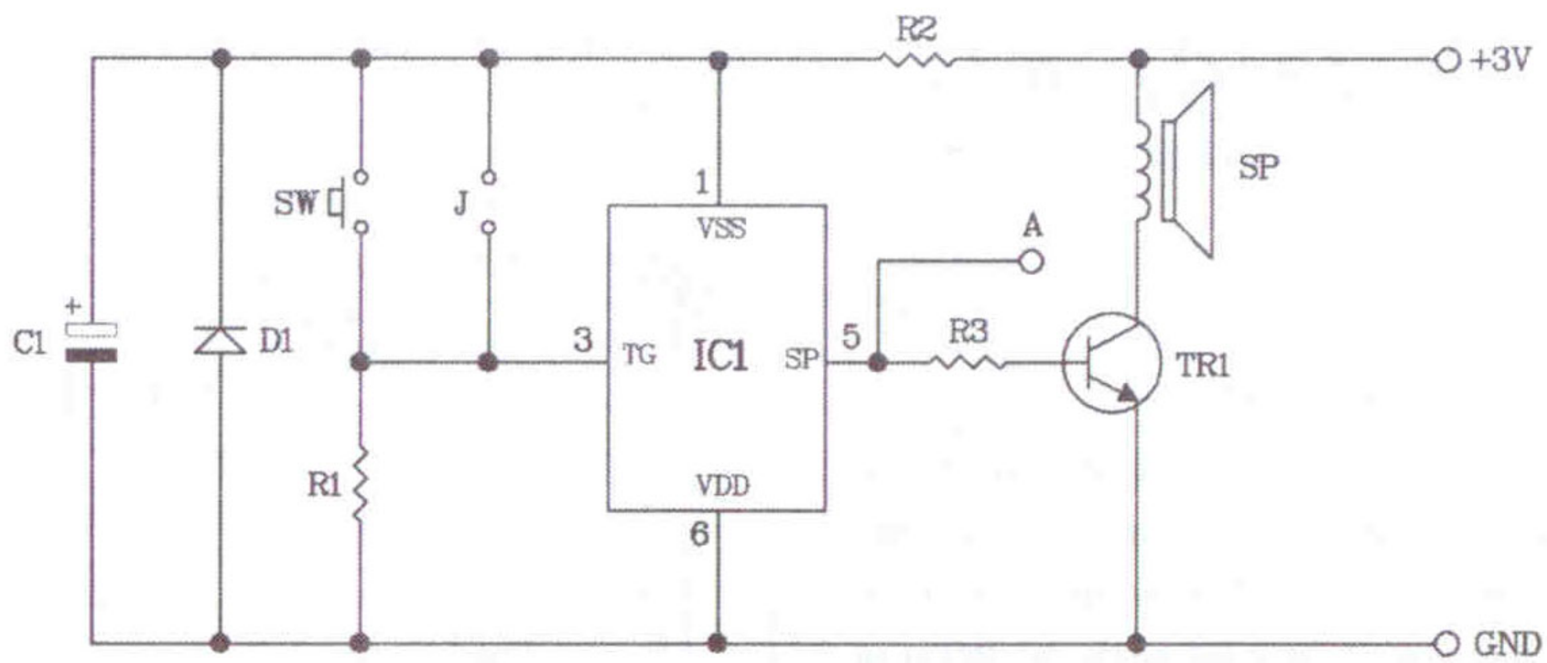
Figure 2. The voice IC digital circuit
