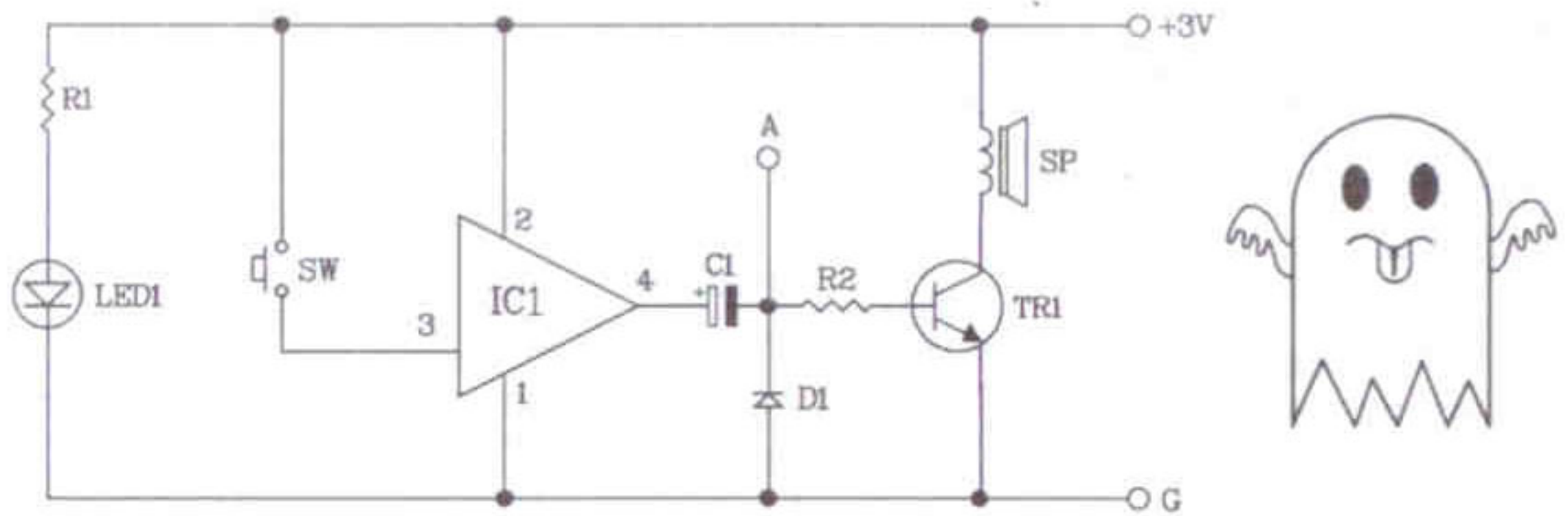
Figure 2. The evil sound circuit
