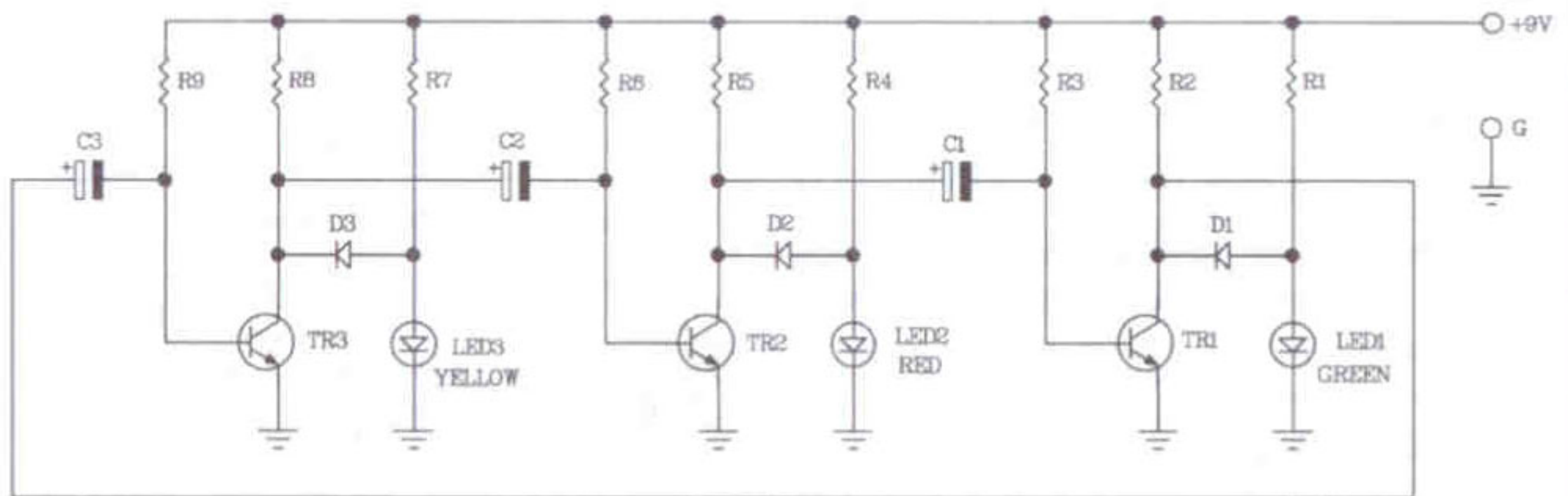
Figure 2. Mini traffic light 3 LED circuit
