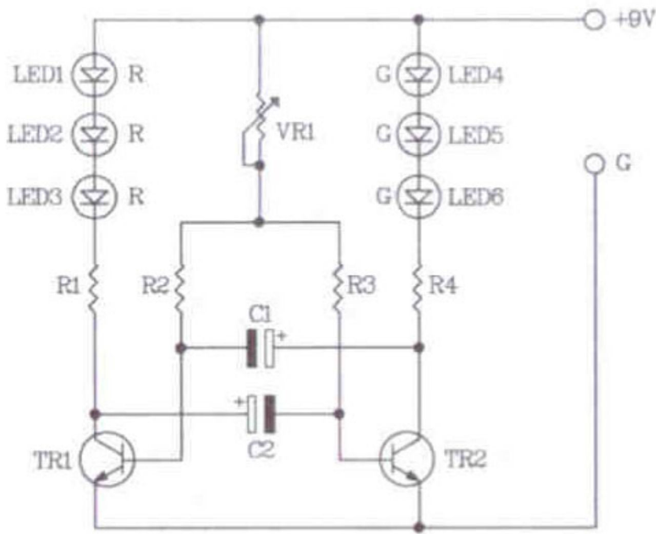
Figure 2. Triangle flasher 6 LED 2 step circuit
