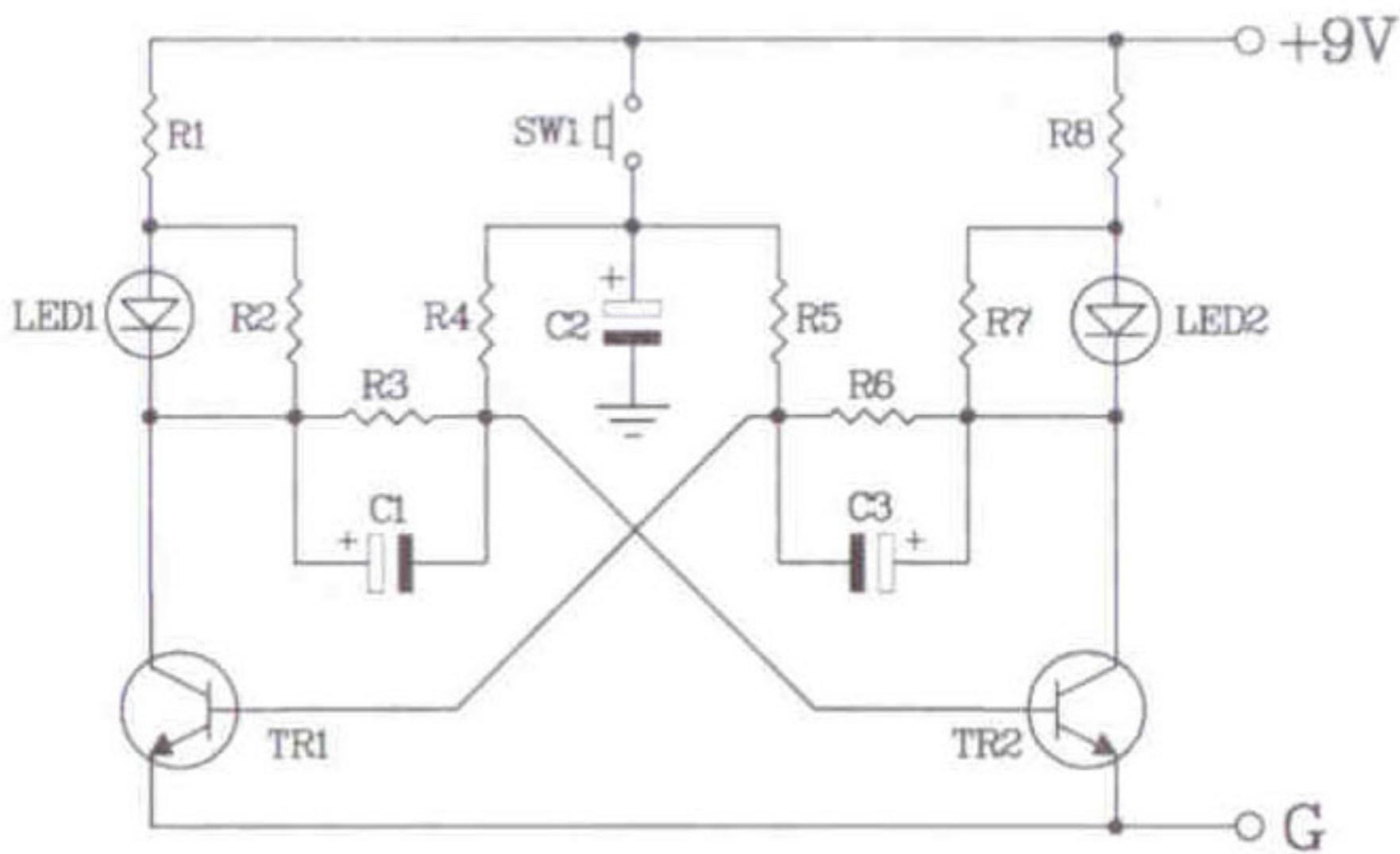
Figure 2. The head or tail games circuit
