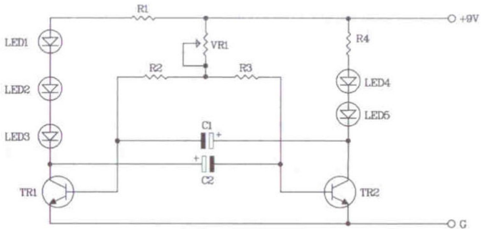
Figure 2. LED flasher 5 dot circuit
