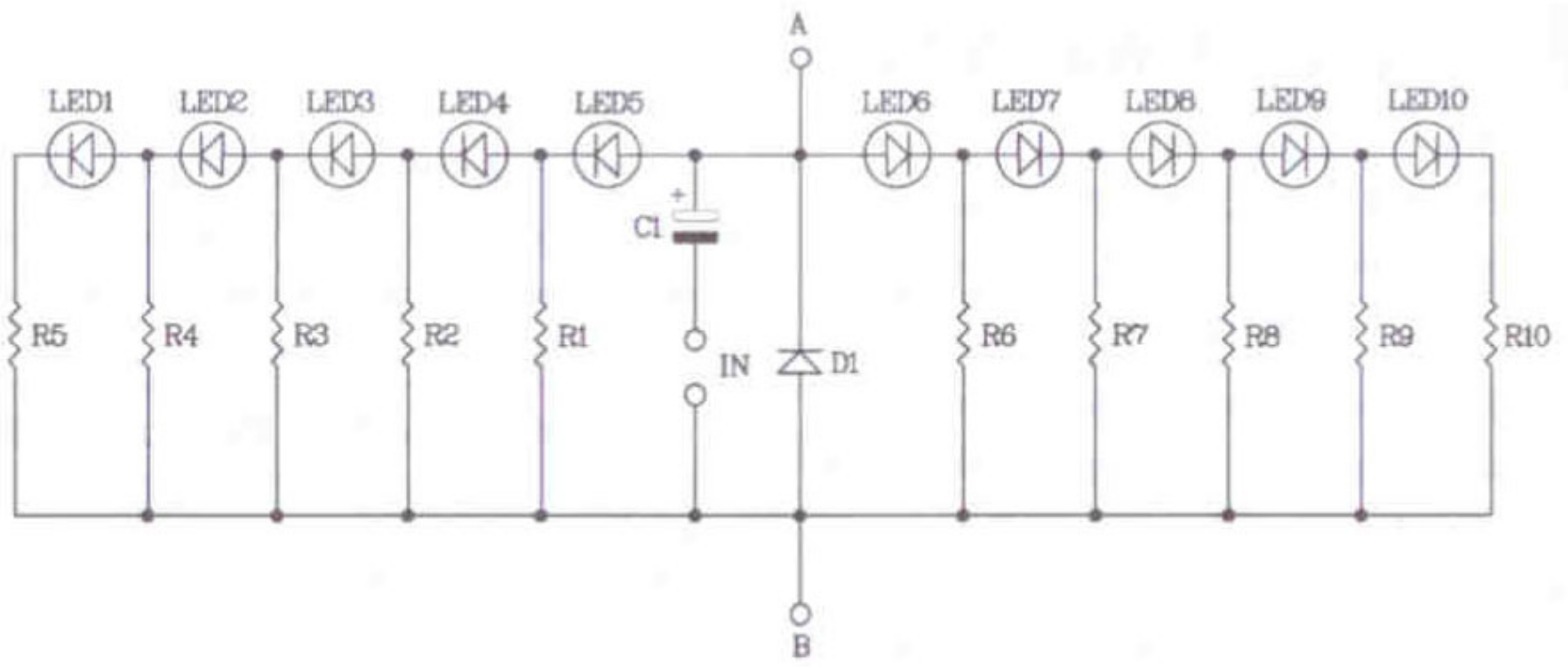
Figure 2. Two way V.U. meter 10 LED circuit
