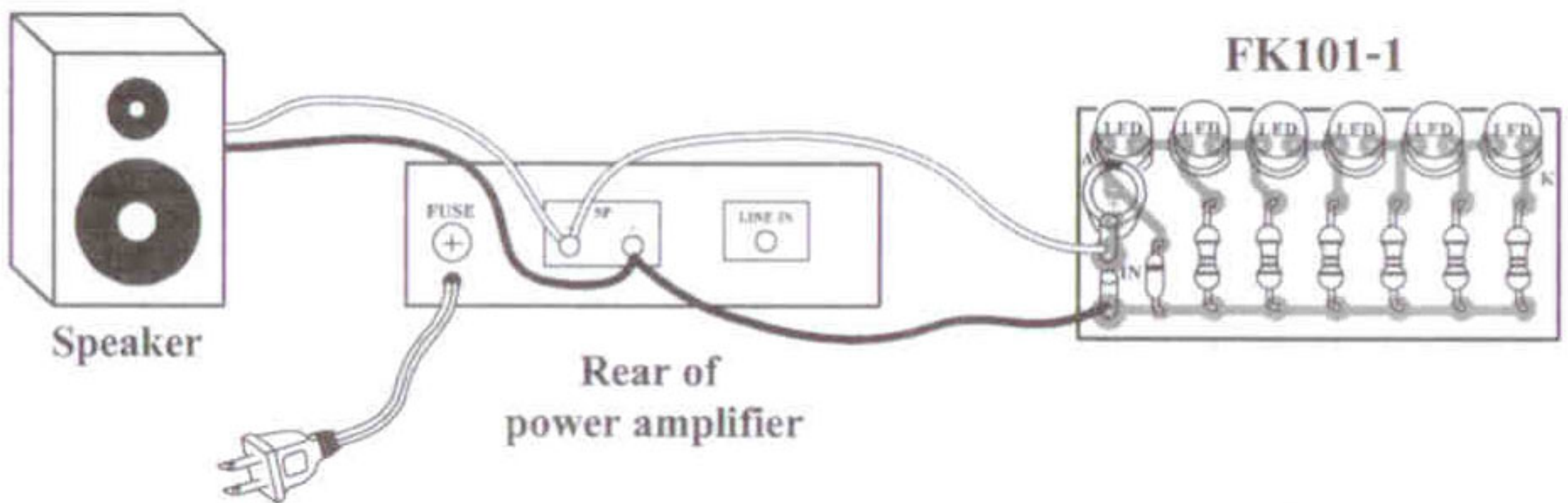
Figure 3. Connections
